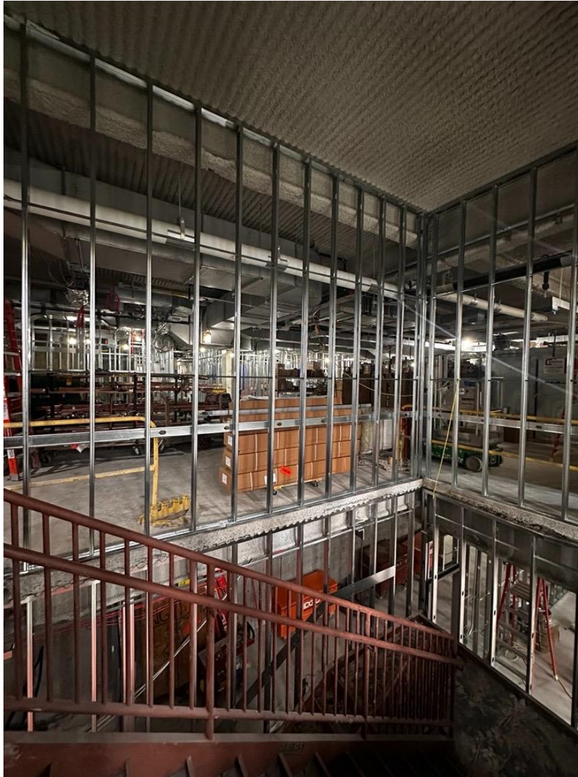
Framework installation around Stair J.
