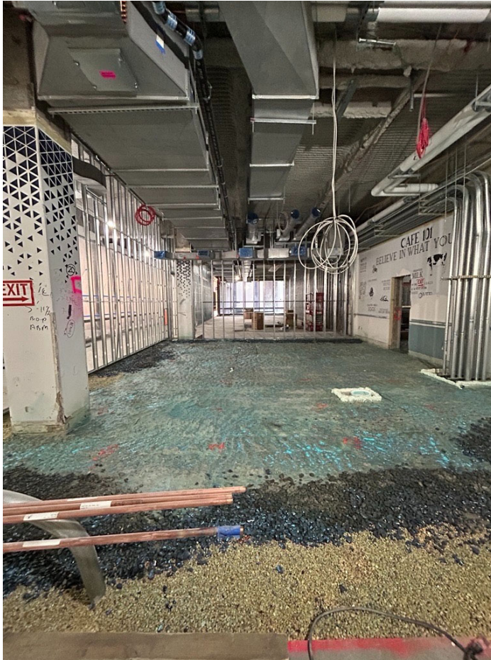
1 st Floor concrete topping slab installation.
