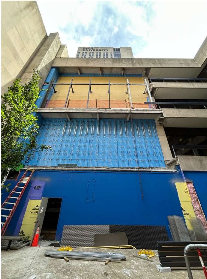
Courtyard Façade progression, support steel being installed for decorative screen.
